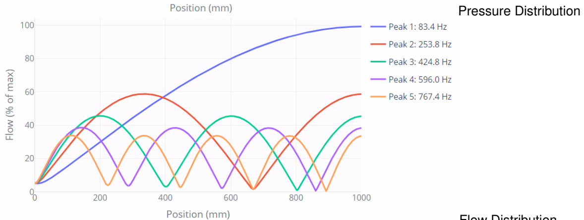
Flow Distribution
