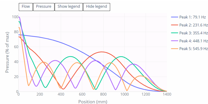
Pressure Distribution
