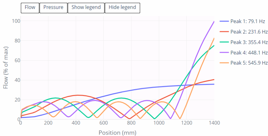
Flow Distribution
