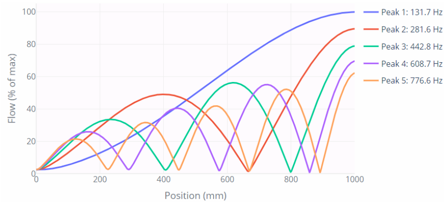
Flow Distribution
